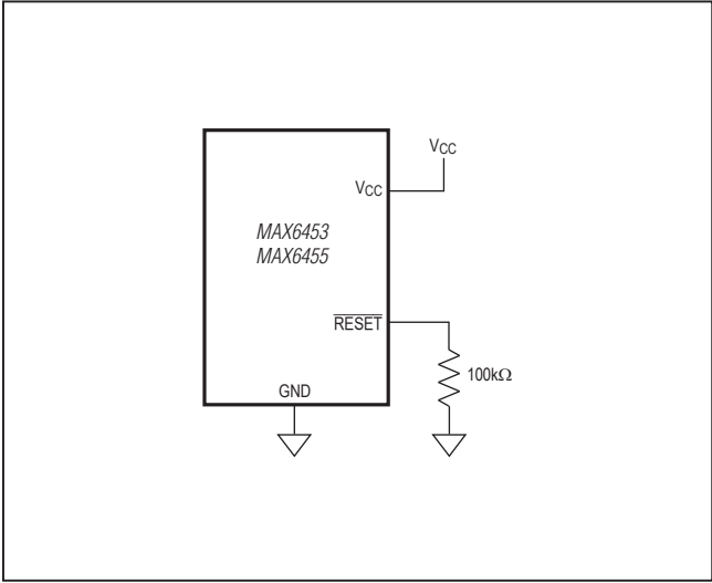
Figure 6. Ensuring \overline{RESET} Valid to V_{CC} = 0
